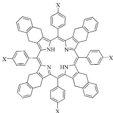
Scheme 4. meso -Tetraaryloctahydro-tetranaphthalo[2,3]porphyrins are isostructural (with respect to inner core without peripheral benzene rings) to porphyrins 5 .
