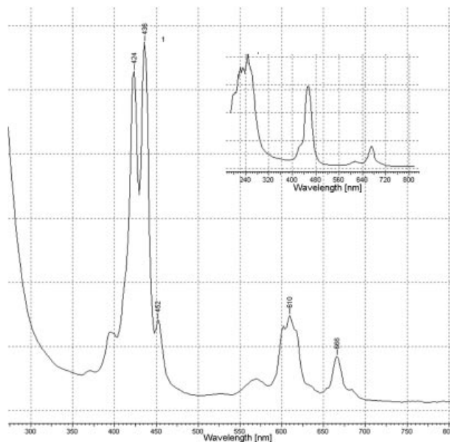
Figure 2. The electronic absorption spectrum of 5,15-diphenyltetrabenzoporphyrin 11 as a free base in \text{CH}_2\text{Cl}_2 (spectrum of dication is shown in the insert).
