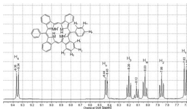
Figure 1. Aromatic portion ( meso protons at 11.01 ppm excluded) of the ^1\text{H} NMR (400 MHz, \text{CDCl}_3 ) of 5,15-diphenyltetrabenzoporphyrin 11 as a dication salt.
