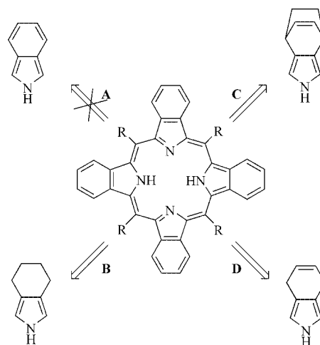
Scheme 1. General routes to tetrabenzoporphyrins.
