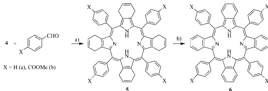
Scheme 3. a) BF 3 ·Et 2 O, CH 2 Cl 2 , room temp., 2 h, then DDQ, room temp., 1 h, 5a (25%), 5b (40%); b) DDQ, toluene, reflux, 5 min, 95%.
