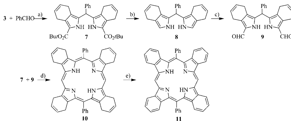
Scheme 5. a) TsOH (cat), n\text{Bu}_4\text{NCl} , \text{CHCl}_3 , room temp., 24 h, 90%; b) TFA, \text{CH}_2\text{Cl}_2 , room temp., 30 min (not isolated); c) \text{CH}(\text{OMe})_3 , TFA, room temp., 30 min, 50% (based on 7 ); d) TFA, \text{CH}_2\text{Cl}_2 , room temp., 21 h, then DDQ, 4 h, 15%; e) DDQ, toluene, reflux, 5 min, >95%.
